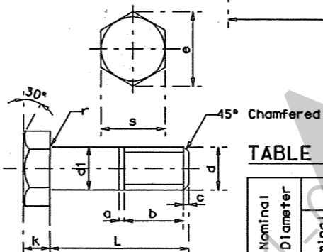
HEX BOLT
