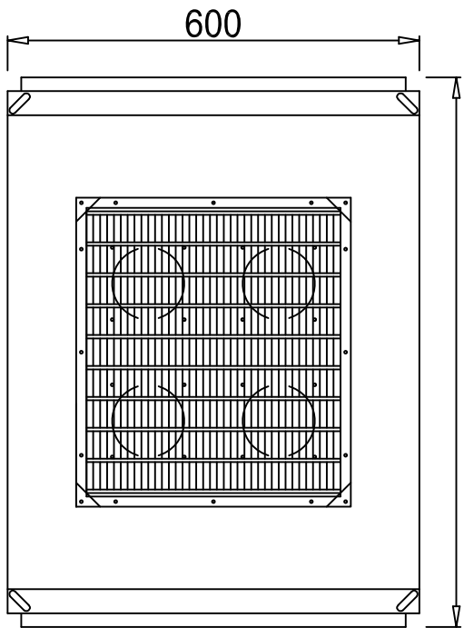
TOP VIEW
