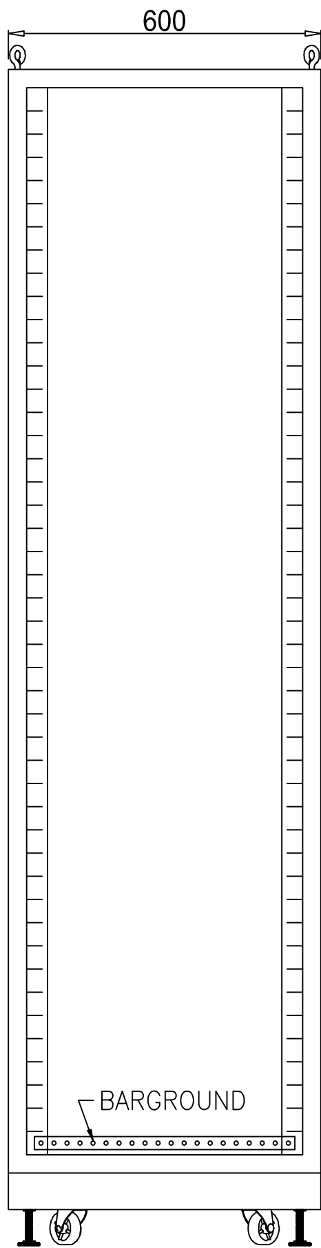
FRONT VIEW WITH OUT DOOR
