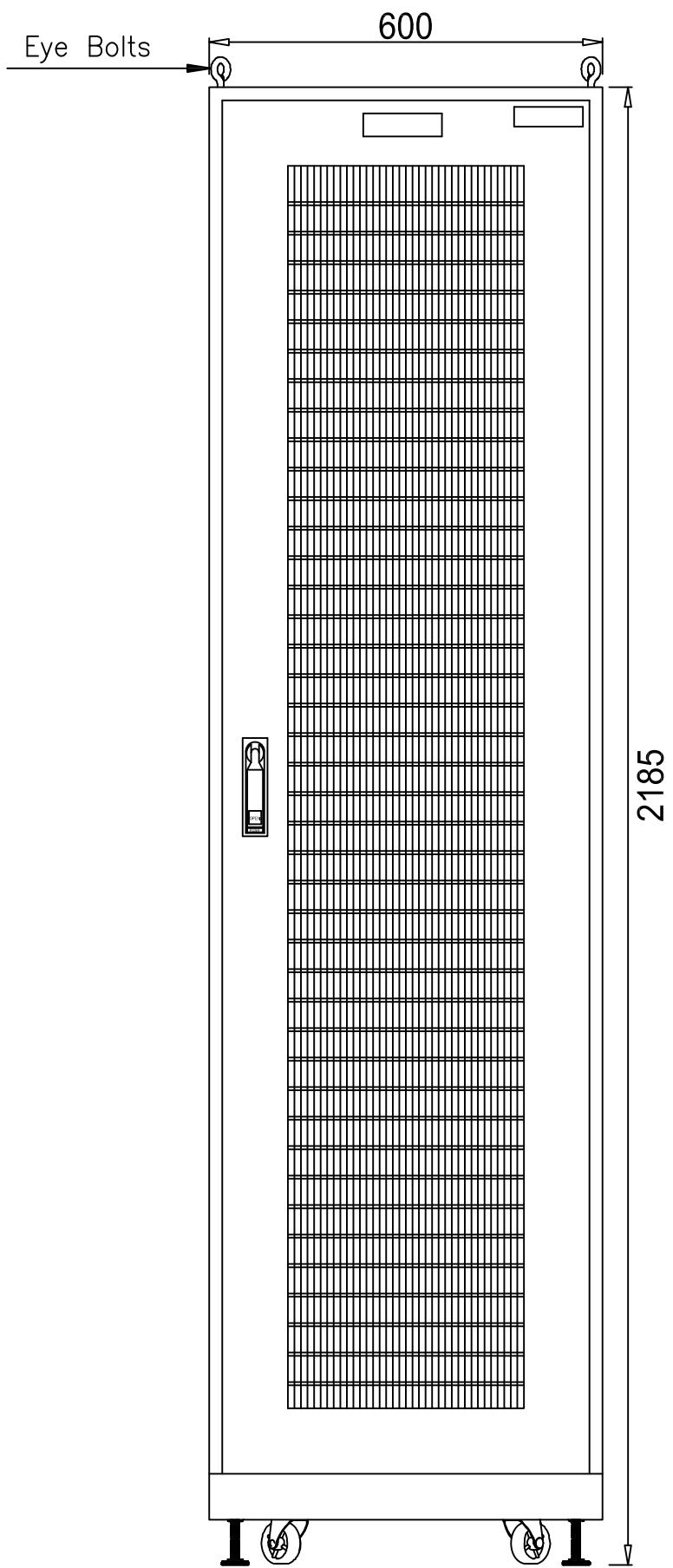
FRONT VIEW
