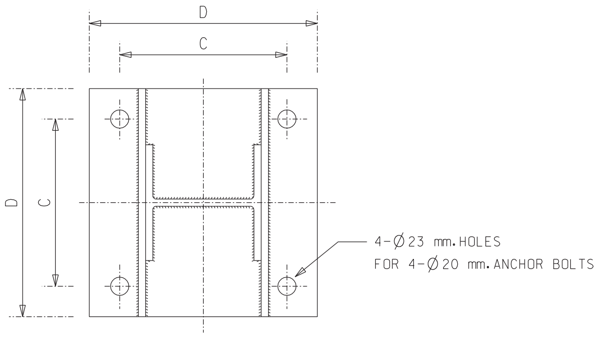
SECTION B-B
