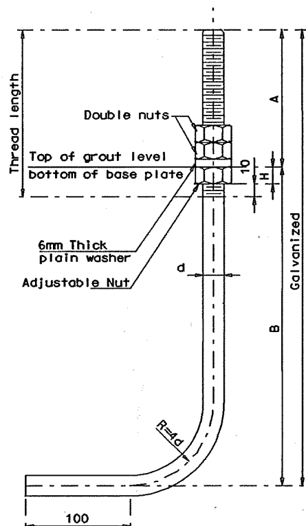
ANCHOR BOLT DETAIL
