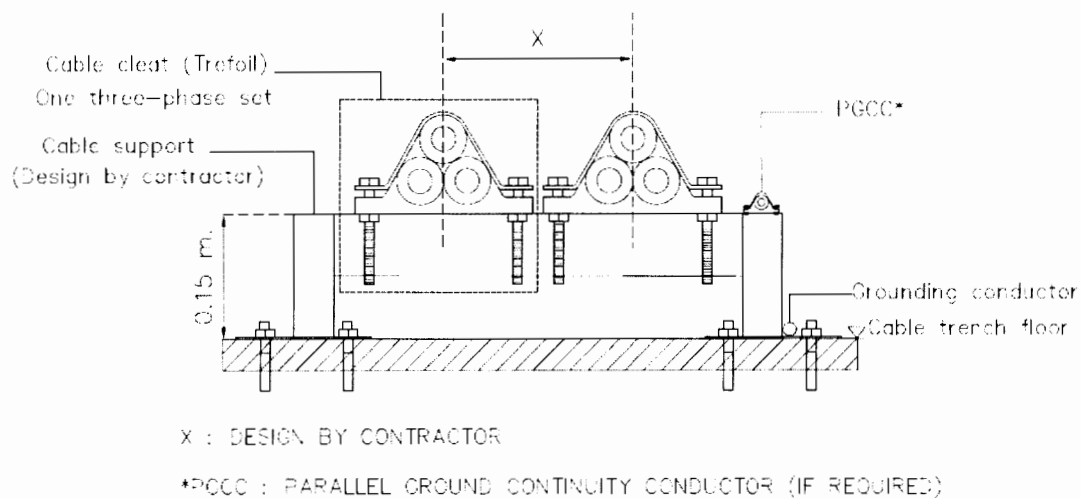
Figure 2: Trefoil Formation
